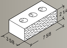
3 \frac{5}{8} \times 2 \frac{1}{4} \times 7 \frac{5}{8} Stretcher
