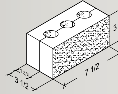
3 \frac{1}{2} \times 3 \frac{1}{2} \times 7 \frac{1}{2} Scored for Soap (Available in 2 & 3-Score.)
