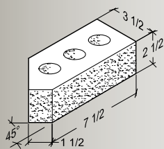
45° Squint
