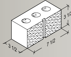
3 \frac{1}{2} \times 3 \frac{1}{2} \times 7 \frac{1}{2} 1-Score
