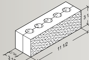
3 \frac{1}{2} \times 3 \frac{1}{2} \times 11 \frac{1}{2} Scored for Soap
