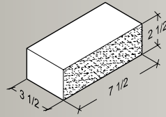
3 \frac{1}{2} \times 2 \frac{1}{2} \times 7 \frac{1}{2} Solid
