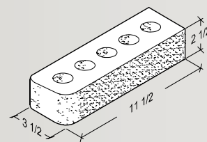
3\frac{1}{2} \times 2\frac{1}{2} \times 11\frac{1}{2} 2 Bullnose Header
