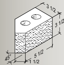
45° Squint
