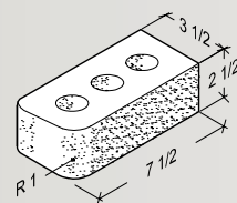
3\frac{1}{2} \times 2\frac{1}{2} \times 7\frac{1}{2} 2 Bullnose Header
