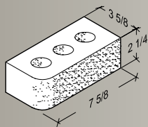
3\frac{5}{8} \times 2\frac{1}{4} \times 7\frac{5}{8} Bullnose
