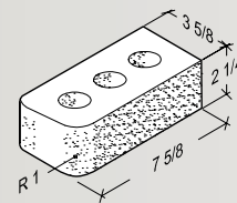
3\frac{5}{8} \times 2\frac{1}{4} \times 7\frac{5}{8} 2 Bullnose Header
