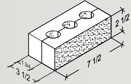
3 \frac{1}{2} \times 2 \frac{1}{2} \times 7 \frac{1}{2} Scored for Soap
