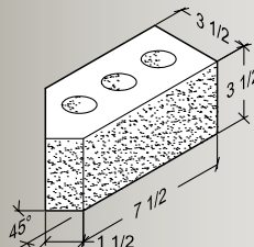
45° Squint
