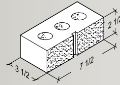
3 \frac{1}{2} \times 2 \frac{1}{2} \times 7 \frac{1}{2} 1-Score (Available in 2 & 3-Score.)
