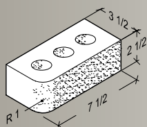
3\frac{1}{2} \times 2\frac{1}{2} \times 7\frac{1}{2} Bullnose
