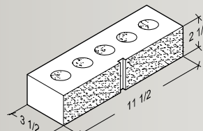
3 \frac{1}{2} \times 2 \frac{1}{2} \times 11 \frac{1}{2} 1-Score (Available in 2 & 3-Score.)
