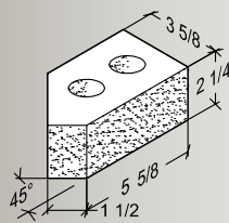
45° Squint
