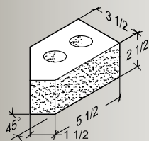
45° Squint
