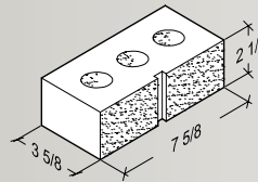
3 \frac{5}{8} \times 2 \frac{1}{4} \times 7 \frac{5}{8} 1-Score (Available in 2 & 3-Score.)
