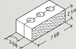
3 \frac{5}{8} \times 2 \frac{1}{4} \times 7 \frac{5}{8} Scored for Soap
