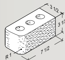
3\frac{1}{2} \times 3\frac{1}{2} \times 7\frac{1}{2} 2 Bullnose Header
