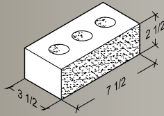
3 \frac{1}{2} \times 2 \frac{1}{2} \times 7 \frac{1}{2} Stretcher
