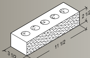
3 \frac{1}{2} \times 2 \frac{1}{2} \times 11 \frac{1}{2} Stretcher
