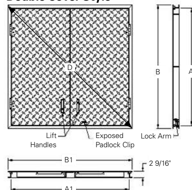
Double Cover Style
