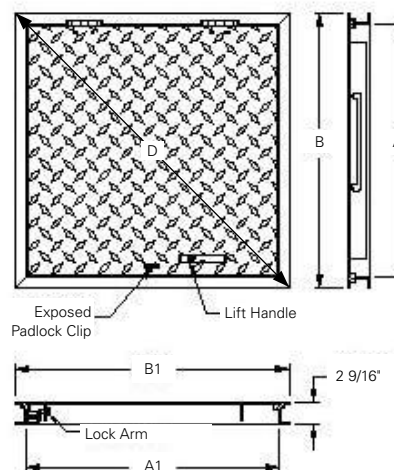
Single Cover Style
