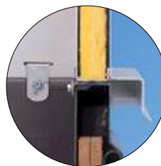
Existing Roof Hatch or Job-Built/Prefab Metal Curbs
