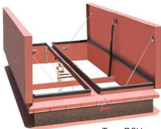
Type DSH Double Leaf c UL US
