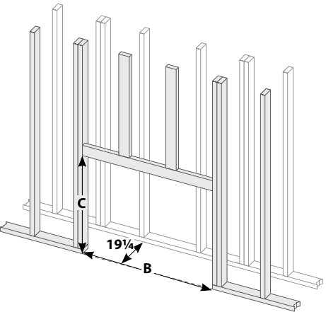
See-through Rough-in Dimensions
