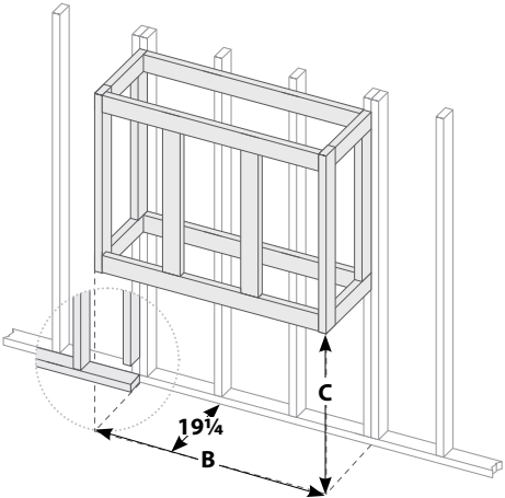
Panorama Rough-in Dimensions
