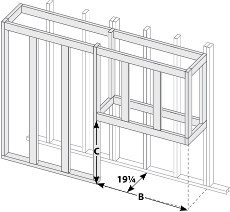
Panorama Rough-in Dimensions
