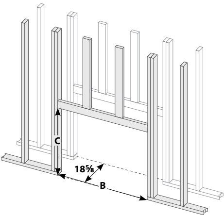
Corner Rough-in Dimensions
